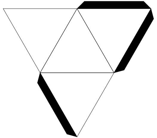
Tetraeder
